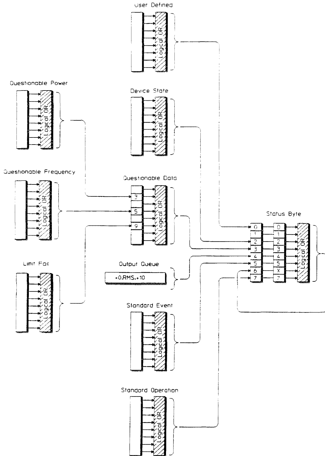
Figure 5-3. HP 3588A Register Summary
